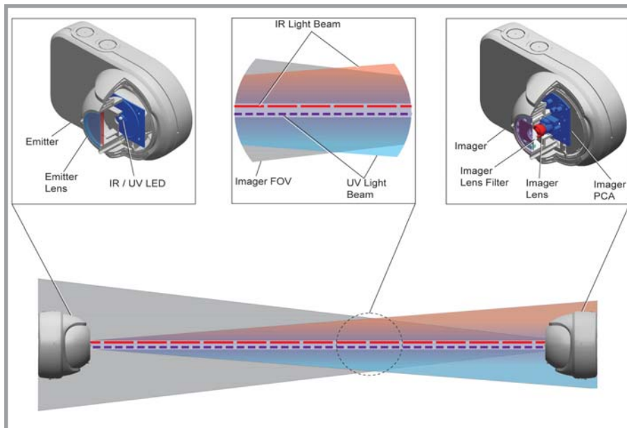
OSID Operational Diagram
